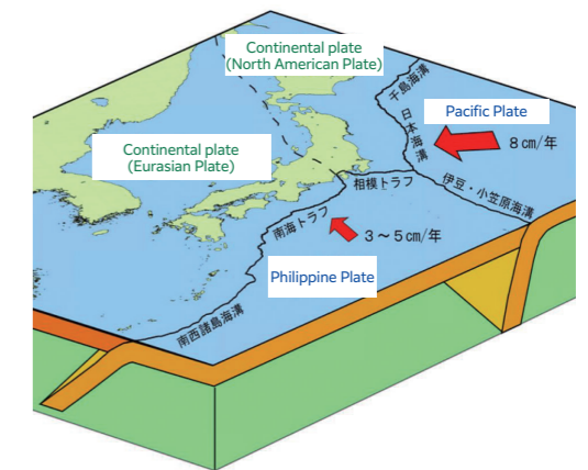
Schematic diagram of tectonic plates around Japan Source: Japan Meteorological Agency
